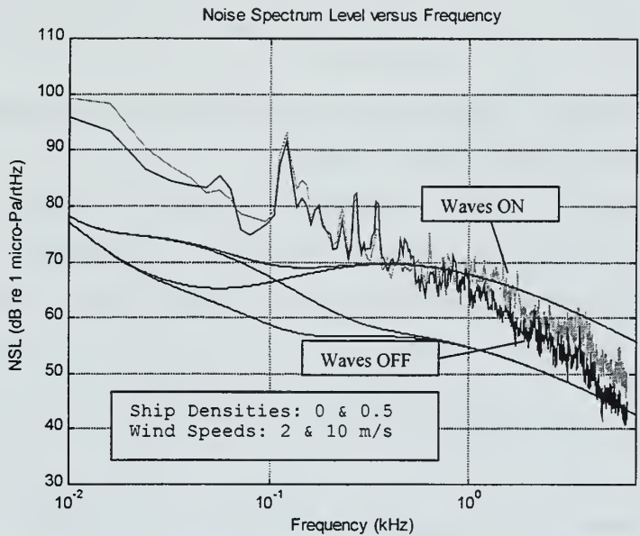
Figure 5.7. Observed 12-Hz-band-average NSL versus frequency in the KFE with the wave machine both on and off. The estimated NSLs are for D=0 and 0.5 , and w=2 and 10 m/s. Total broadband ( 0-6.4 kHz) NLs are 114 dB and 112 dB re 1 \mu\text{Pa} for the KFE with waves off and on, respectively.
